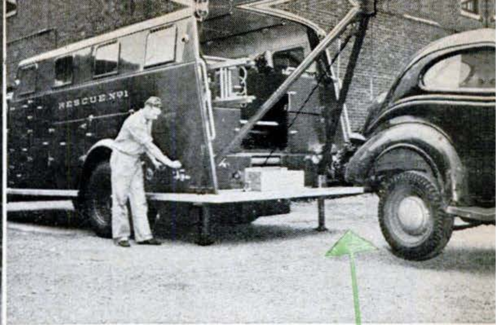
RUGGED HOIST , carried inside truck and set up at emergency scene, lifts weights off people pinned under them. Heavy jacks let down from truck's rear end take the load.
